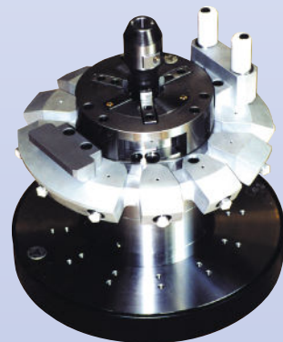
Centering and stirruping chuck for turning
