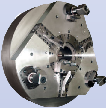
No-distortion chuck for carbon fiber bike wheels clamping
